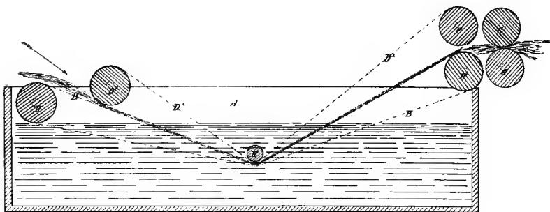
FIG. 33.—Washing Trough.
