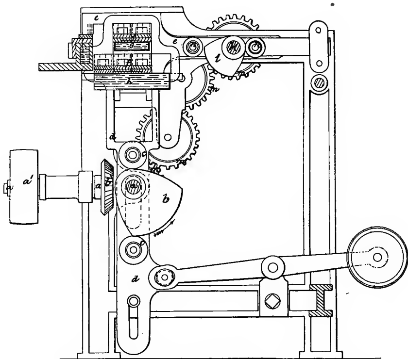
FIG. 51.—End View.
