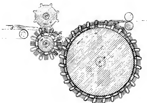
FIG. 34.—Feed Rollers.
