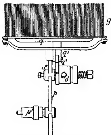
FIG. 27.—The Carrying Comb.
