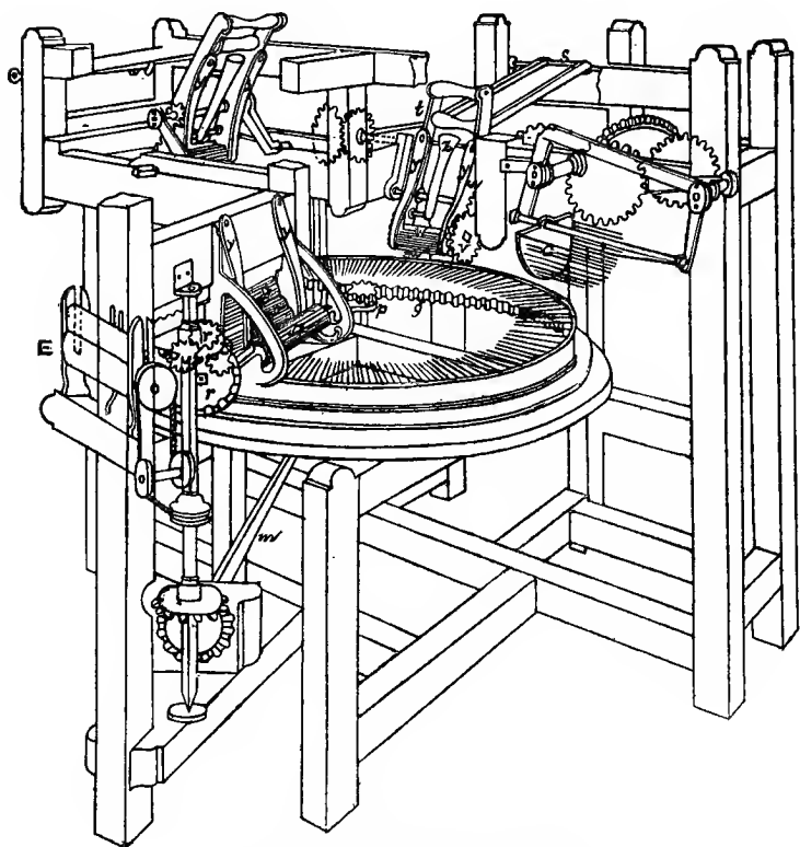
FIG. 5.—Dr. Cartwright's "Big Ben."
