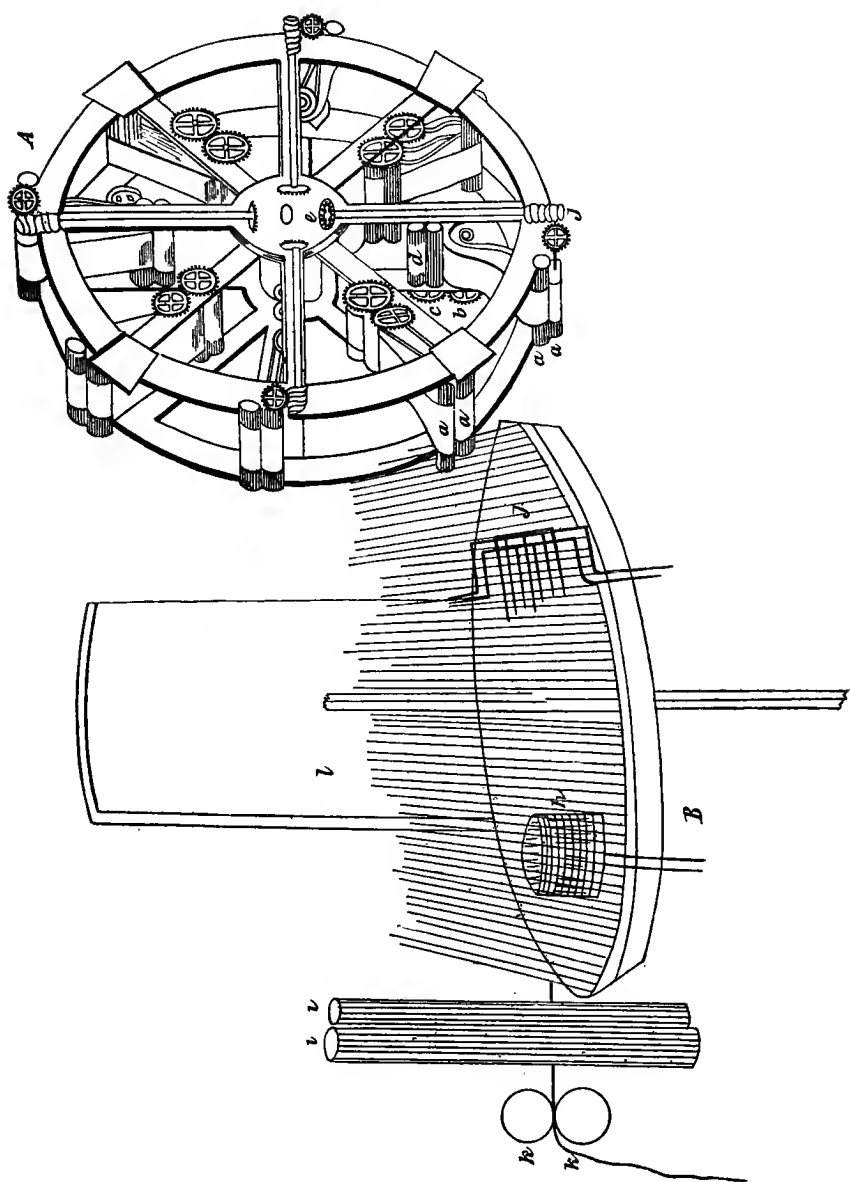
FIG. 3.—Dr. Cartwright's "Big Ben."
