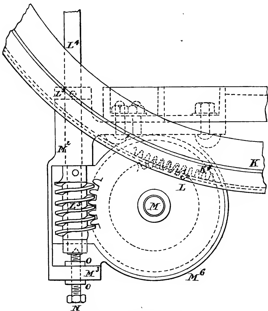
FIG. 66.—Motion to Circle of Comb Teeth.
