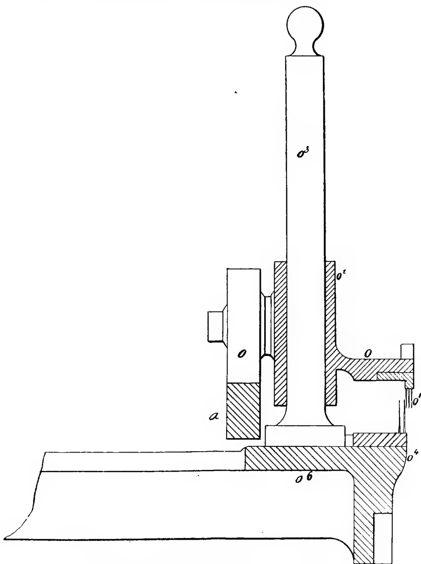
FIG. 61.—Section of Conductors to “nacteur” Combs.
