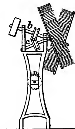
FIG. 11.—Enlarged Diagram.
