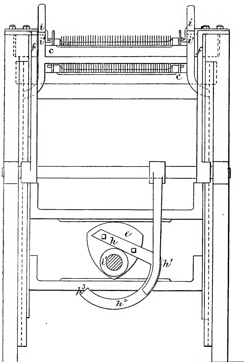
FIG. 39.—Portion of front view of Machine of 5th May, 1856.
