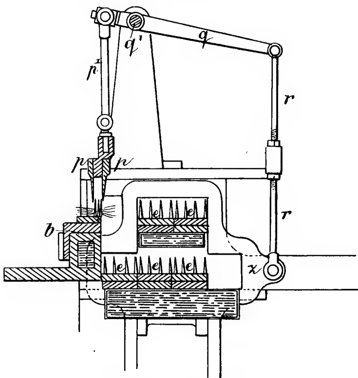
FIG. 55.—View of Motion.
