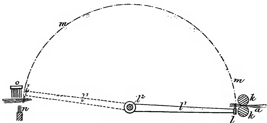
FIG. 54.—Feed Rollers.
