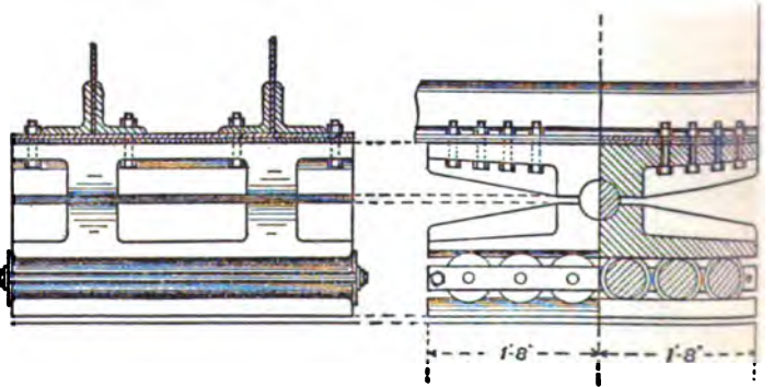
FIG. 14.—Roller Bed of a Girder.
