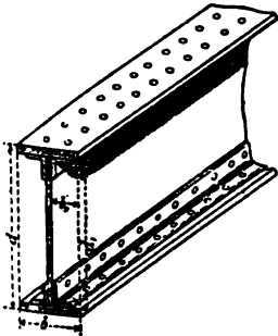
FIG. 15.—Flanged Girder.
