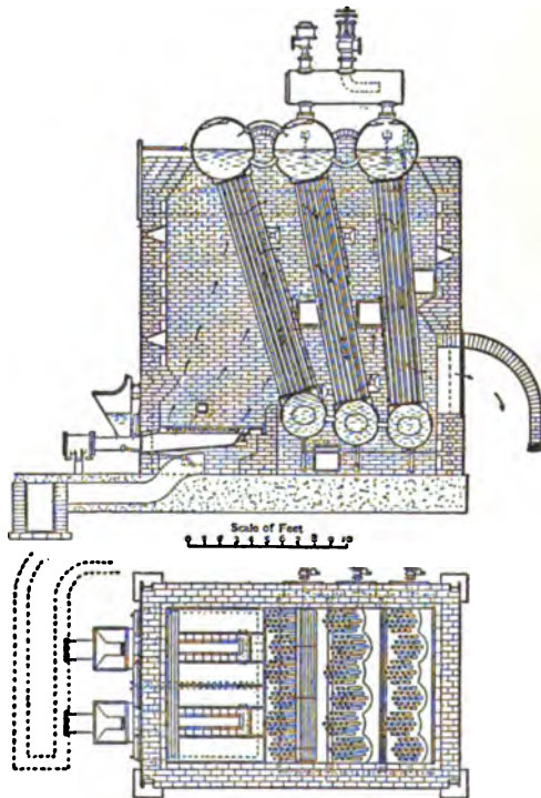
FIG. 13.—Woodson Boiler (Messrs Clarke, Chapman & Co.).
