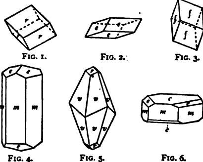
FIGS. 1-6.—Crystals of Calcite.
