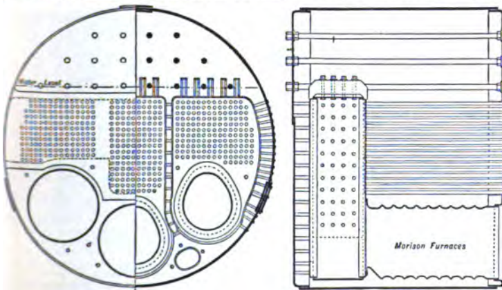
FIG. 7.—Single-ended Marine Boiler.
