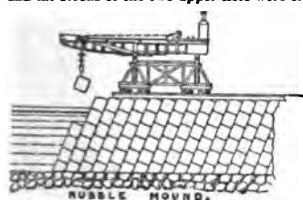
FIG. 10.—Colombo North-West Breakwater with Titan Crane.
