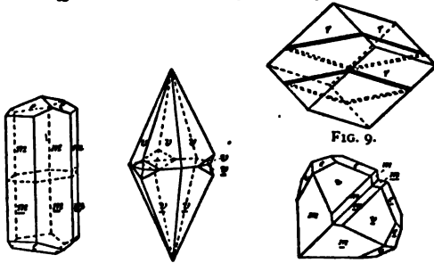
FIG. 7. FIG. 8. FIG. 9. FIG. 7-10.—Twinned Crystals of Calcite.
