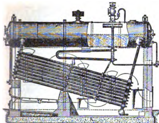
FIG. 11.—Babcock & Wilcox Water-tube Boiler fitted with Superheaters.
