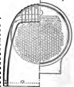
Fig. 10.—Express Locomotive Boiler, with widened fire-box (Great Northern Railway, England).
