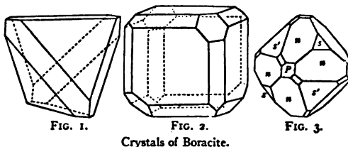
Crystals of Boracite.
