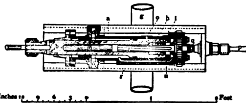
FIGS. 4 and 5.—Darlington's Rock Drill.
