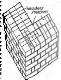
In this and following illustrations of bond in brickwork the position of bricks in the second course is indicated by dashed lines.
