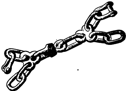
FIG. 2.—Mooring Swivel.
