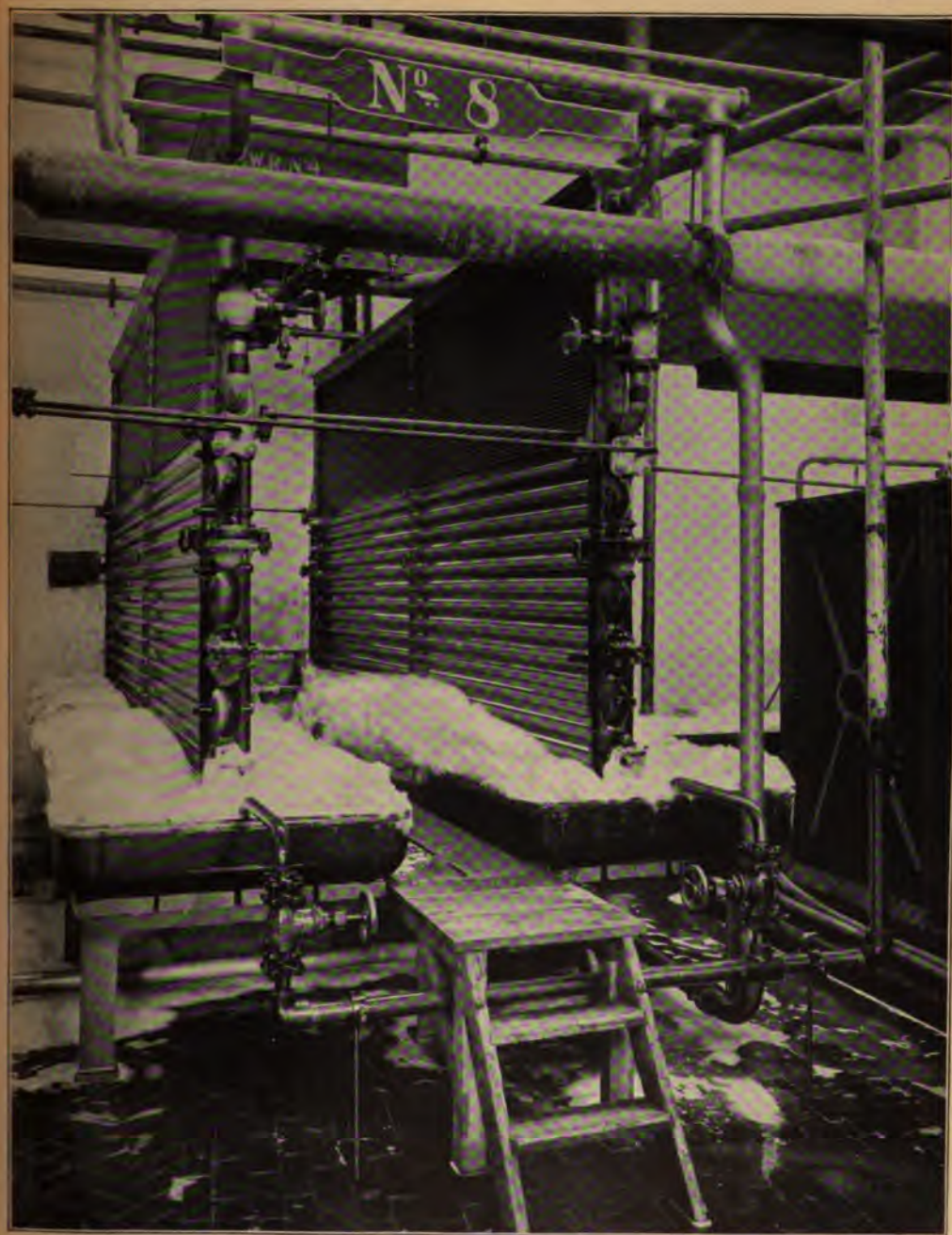
Fig. 5.—Refrigerators in "Lager" Brewery of Messrs. Allsopp. The hot wort trickles over the outside of the series of pipes, and is cooled by the cold water which circulates in them. From the shallow collecting trays the cooled wort is conducted to the fermenting backs.
