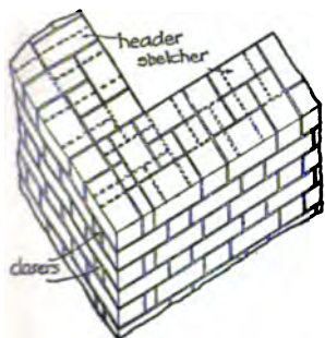
FIG. 6.—Flemish Bond.
