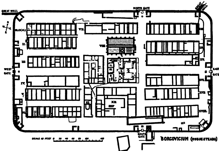
FIG. 1.—Plan of Housesteads (Borcovium) on Hadrian's Wall.
