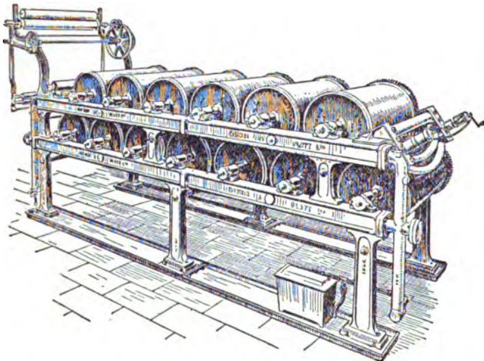
FIG. 8.—Mather & Platt's Horizontal Drying Machine.
