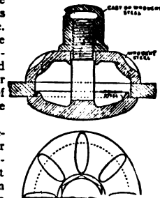
FIG. 18.—Handhole Fittings.
