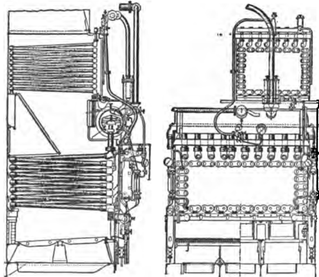
FIG. 14.—Belleville Boiler.
