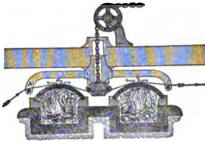
FIG. 2.—Section of Singe-stove.
