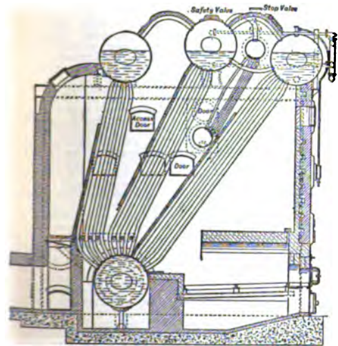
FIG. 12.—Stirling Water-tube Boiler.
