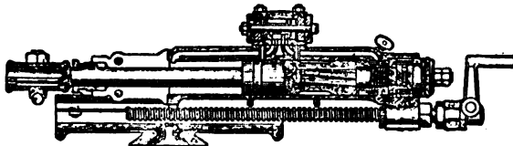
FIG. 6.—New Ingersoll Drill.
