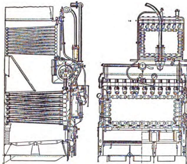
FIG. 14.—Belleville Boiler.
