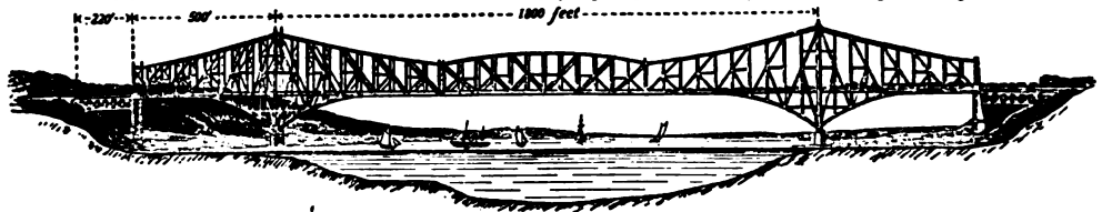
FIG. 25.—Quebec Bridge (original design).
