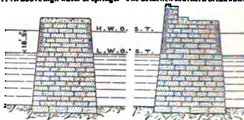
Dover Breakwater.
