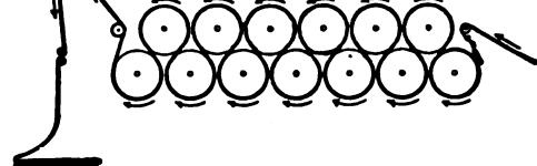
FIG. 9.—Diagram showing the Horizontal Drying Machine threaded with Cloth.
