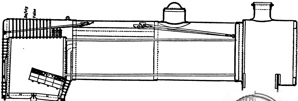
Fig. 10.—Express Locomotive Boiler, with widened fire-box (Great Northern Railway, England).
