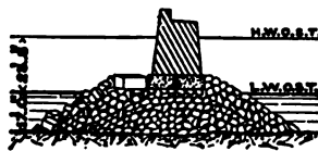
FIG. 8.—Havre Breakwater.
