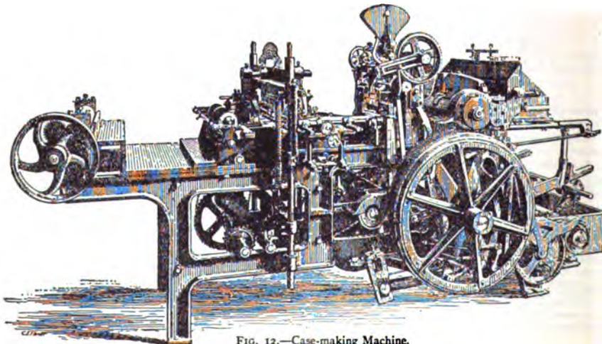
FIG. 12.—Case-making Machine.
