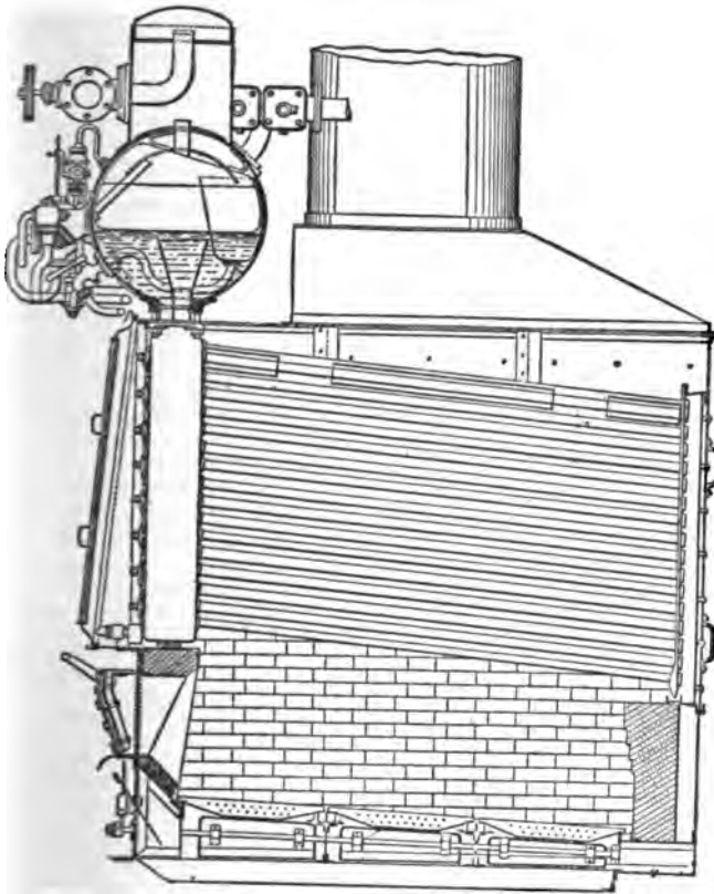
FIG. 15.—Niclausse Boiler—transverse section.
