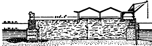
FIG. 16.—Zebrugge Harbour Breakwater with Quay.
