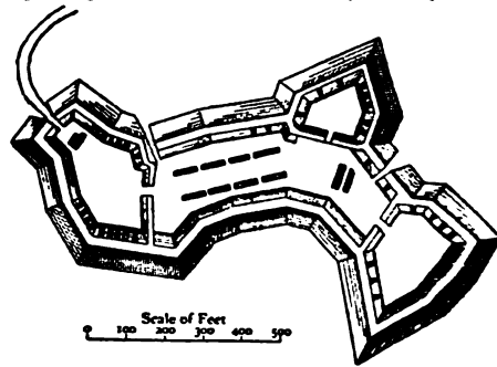
FIG. 76.—Torres Vedras Works.
