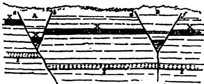
FIG. 10.—Trough faults.
