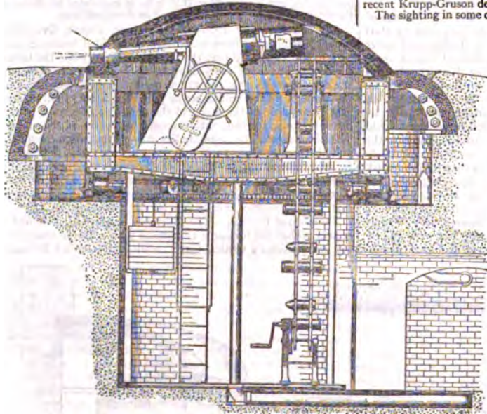
FIG. 56.—Cupola for 6-in. gun (Friedr. Krupp A.G.).
