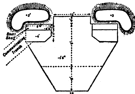
From M.H. Engineering: Field Defences , by permission of the Controller H.M. Stationary Office.
