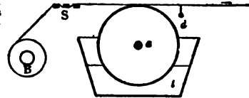
FIG. 1.—Principle of Back-Starching Machine.
