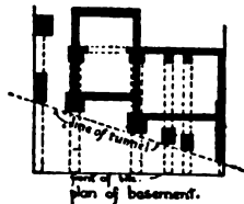
FIG. 13.—Cantilever Foundation over Railway Tunnel
