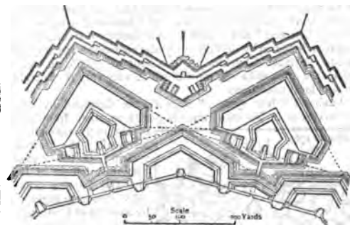
FIG. 23.—Speckle's Reinforced Trace.
