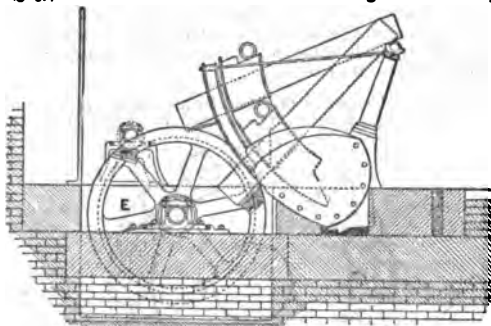
FIG. 5.—Milling Stocks.
