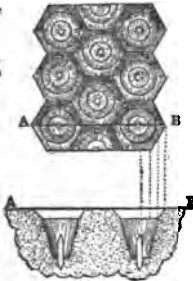
FIG. 95.—Plan and section of Trou-de-loup
